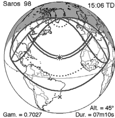
Annular Saros 98 1125 Dec 26 15:06 TD
