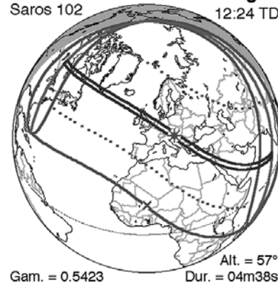
Total Saros 102 1133 Aug 02 12:24 TD
